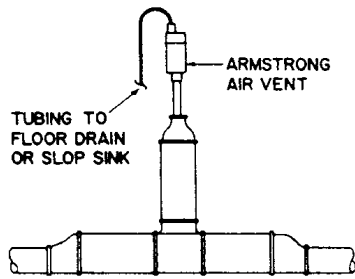
Fig. 2-1. Installation of automatic air vent on piping.
