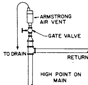
Fig. 2-2. Installation of automatic air vent on high point of system.
