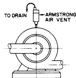
Fig. 2-6. Venting air from a centrifugal pump.
