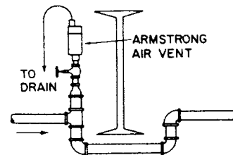
Fig. 2-3. Installation of automatic air vent on loop in piping.
